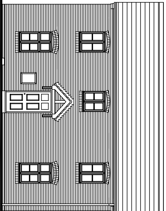
Front Elevation
