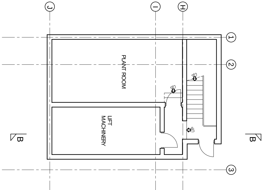
FOURTH FLOOR LAYOUT TOTAL FLOOR AREA 52m²
