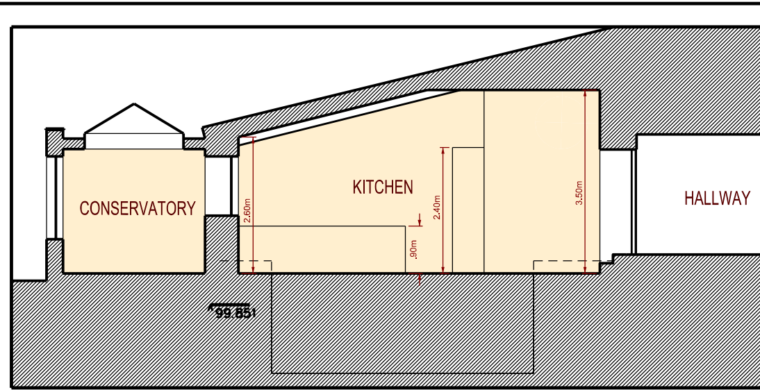
Cross Section
