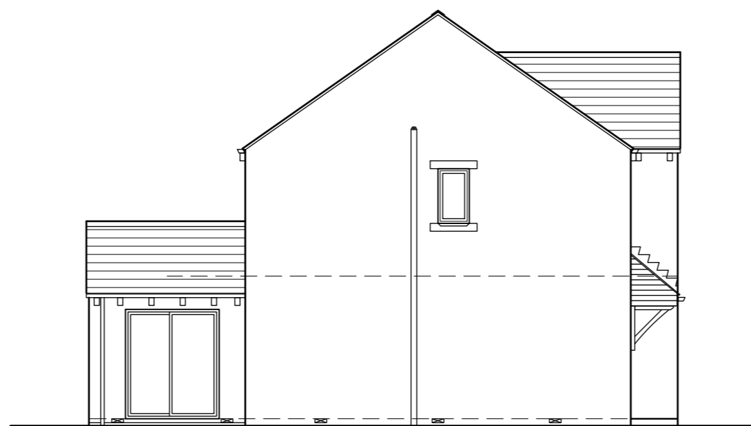
East Elevation
