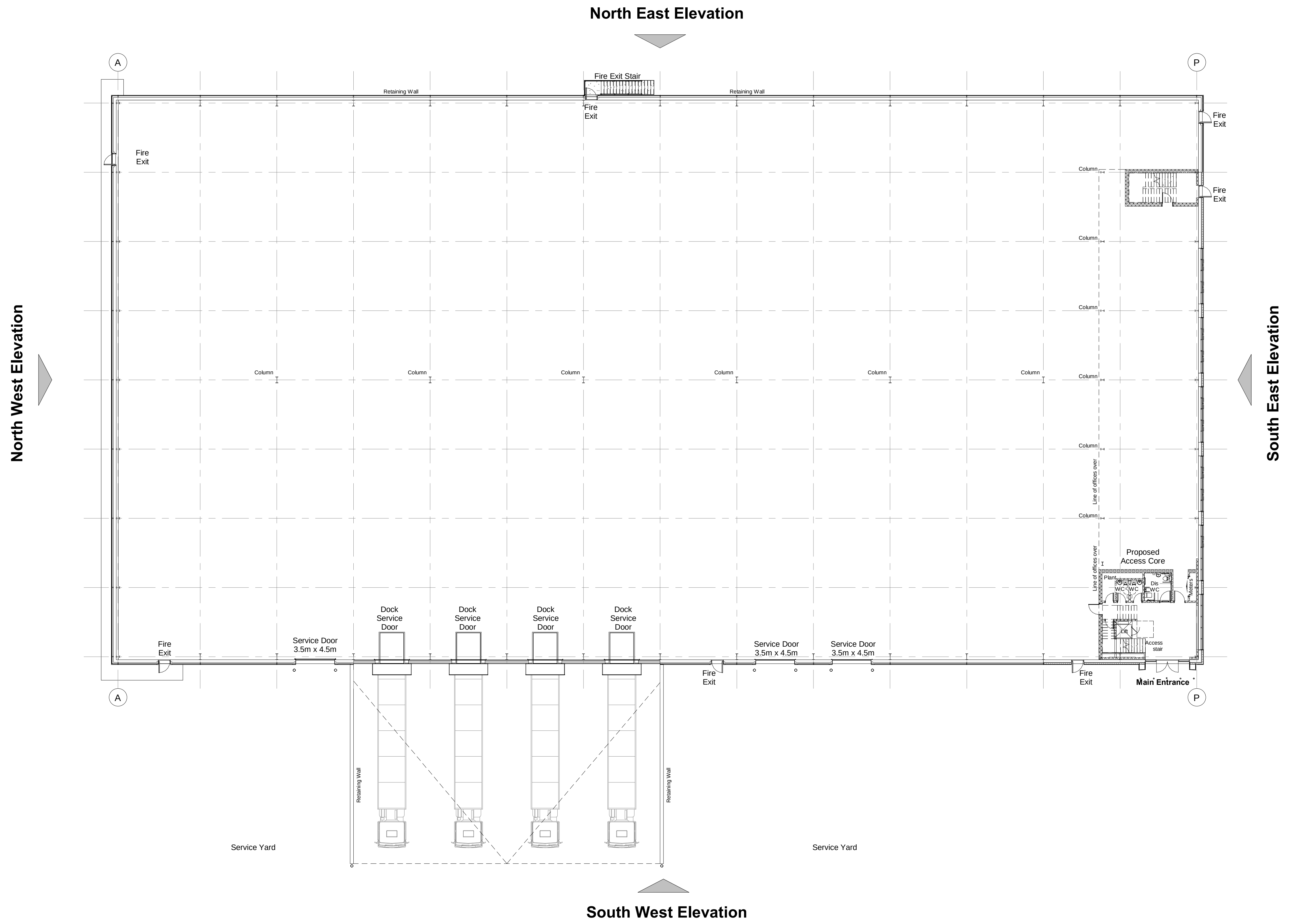
Proposed Ground Floor 1 : 200
