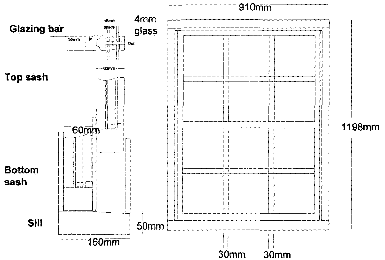
SASH WINDOW DESIGN DETAILS
