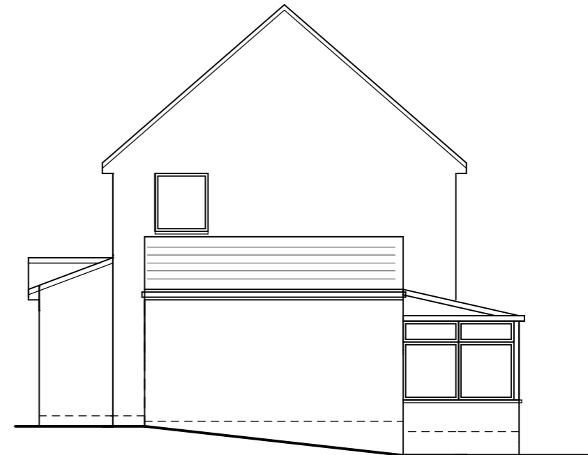
right side (west) elevation
