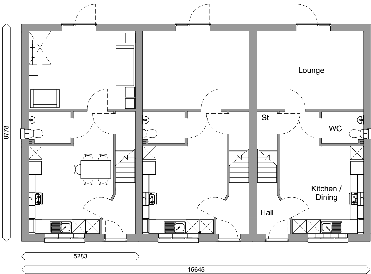
Ground Floor. 1 : 100
