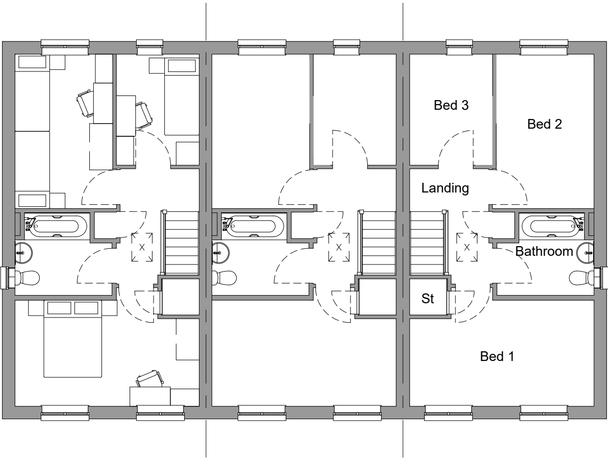
First Floor. 1 : 100
