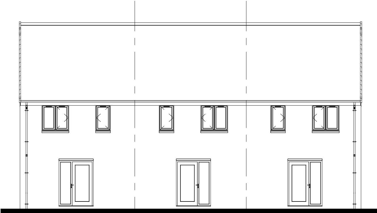
Rear Elevation.
