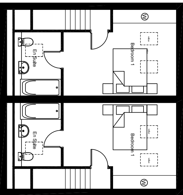
Proposed Second Floor Plan- Plot 1-8 1:100
