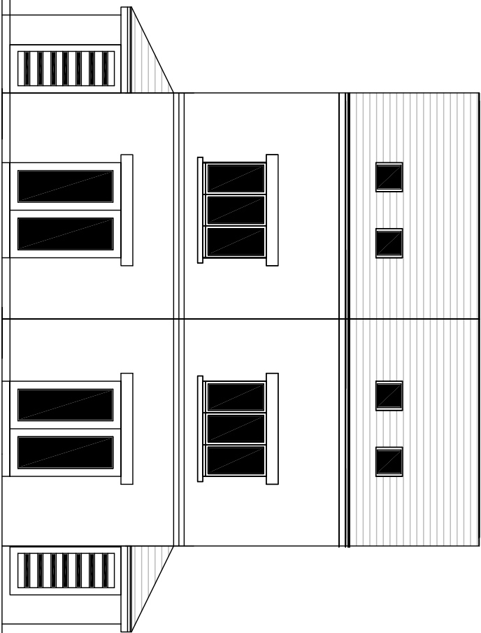
Proposed Rear Elevation- Plot 1-8 1:100
