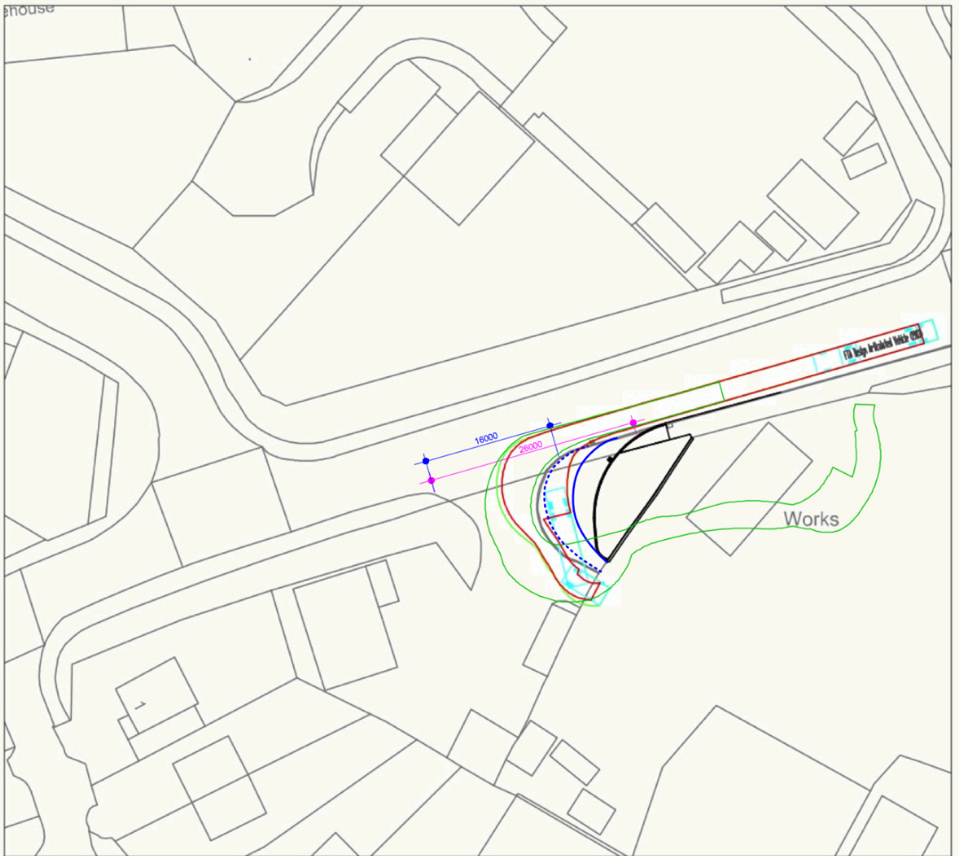
Articulated Vehicle left turn 1:500
