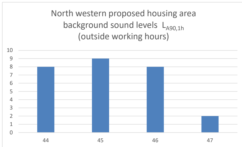
Figure 3 North western proposed housing area background sound levels (outside working hours)
