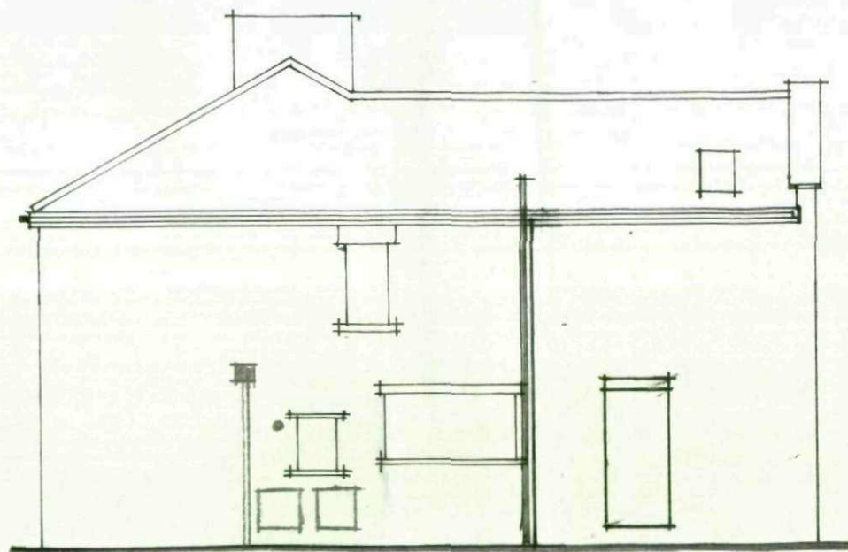
SIDE ELEVATION (FROM ADJ BUILDING & DRIVE.)
