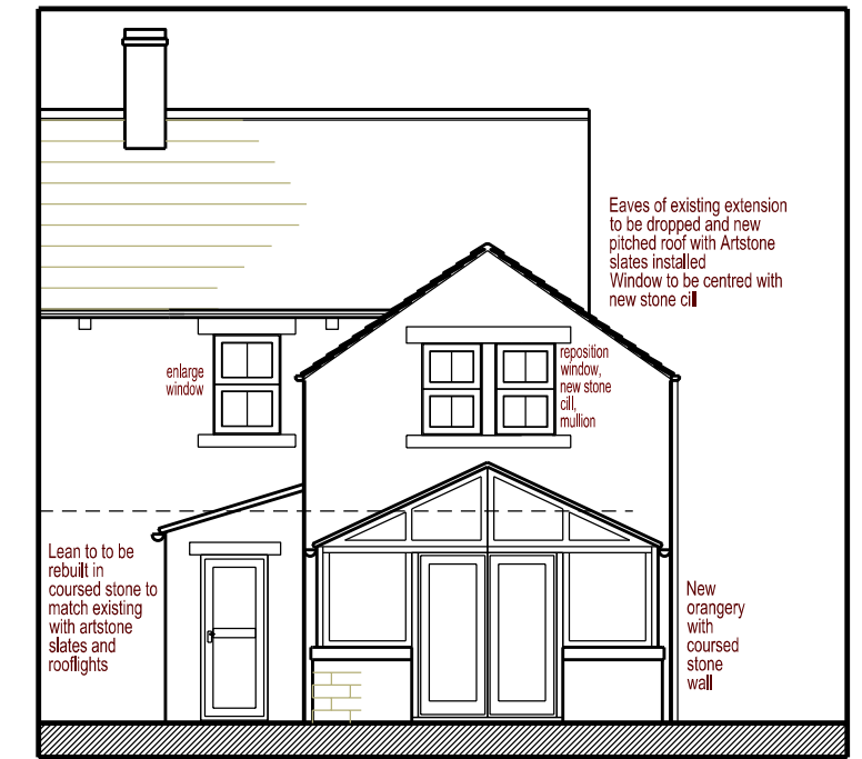
South Elevation - Proposed
