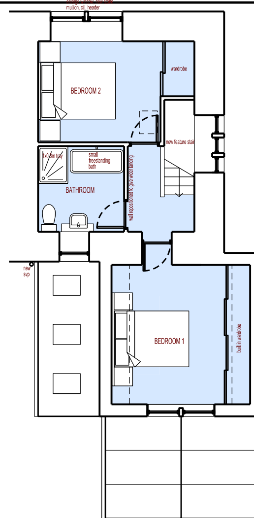
First Floor Plan - Proposed
