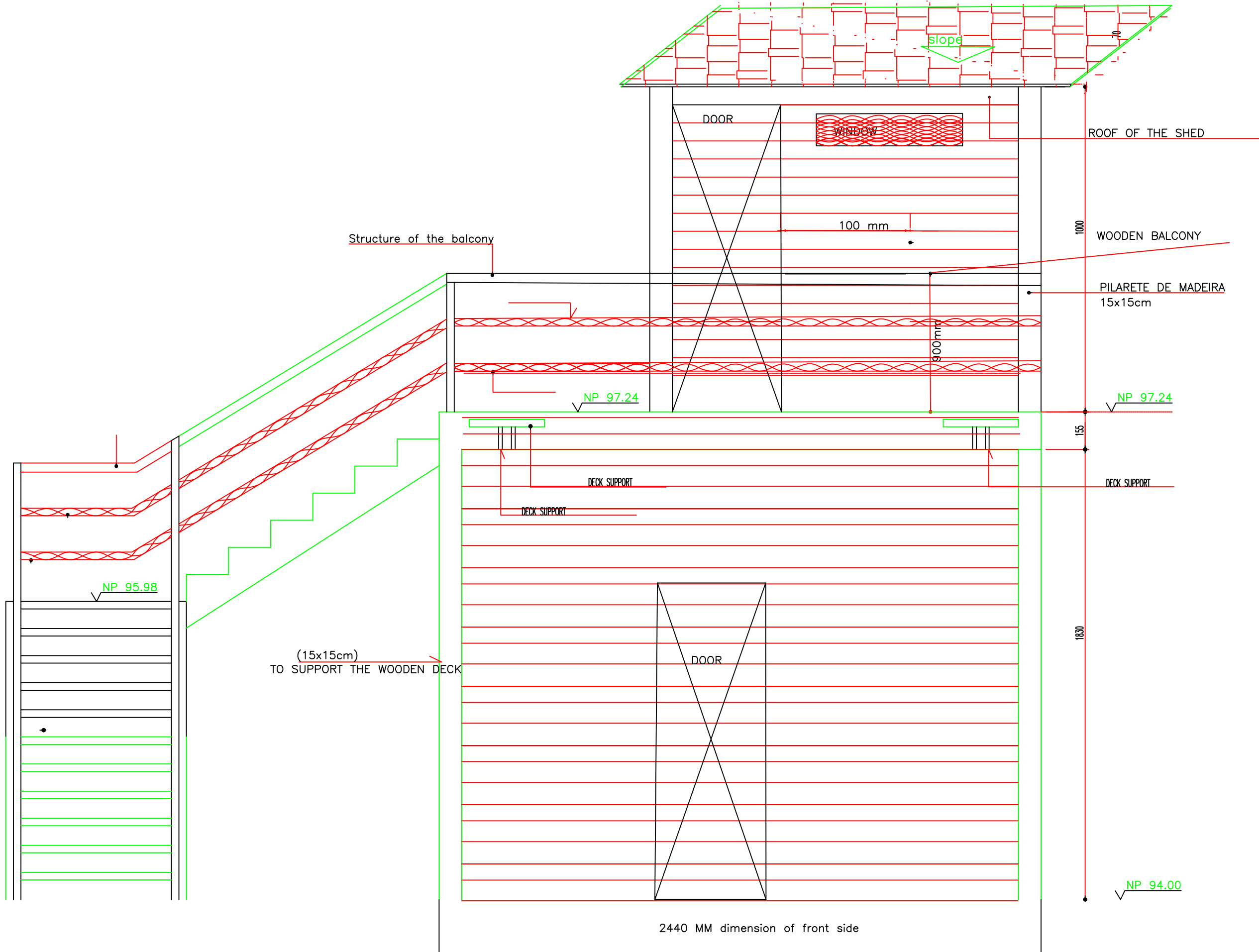
Drawing.1 – Elevation "A" – Front View ESC: 1:25
