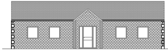
SIDE ELEVATION VIEW ON 'D'
