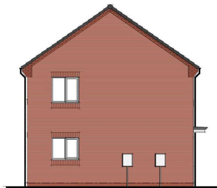
L.H. SIDE ELEVATION.
