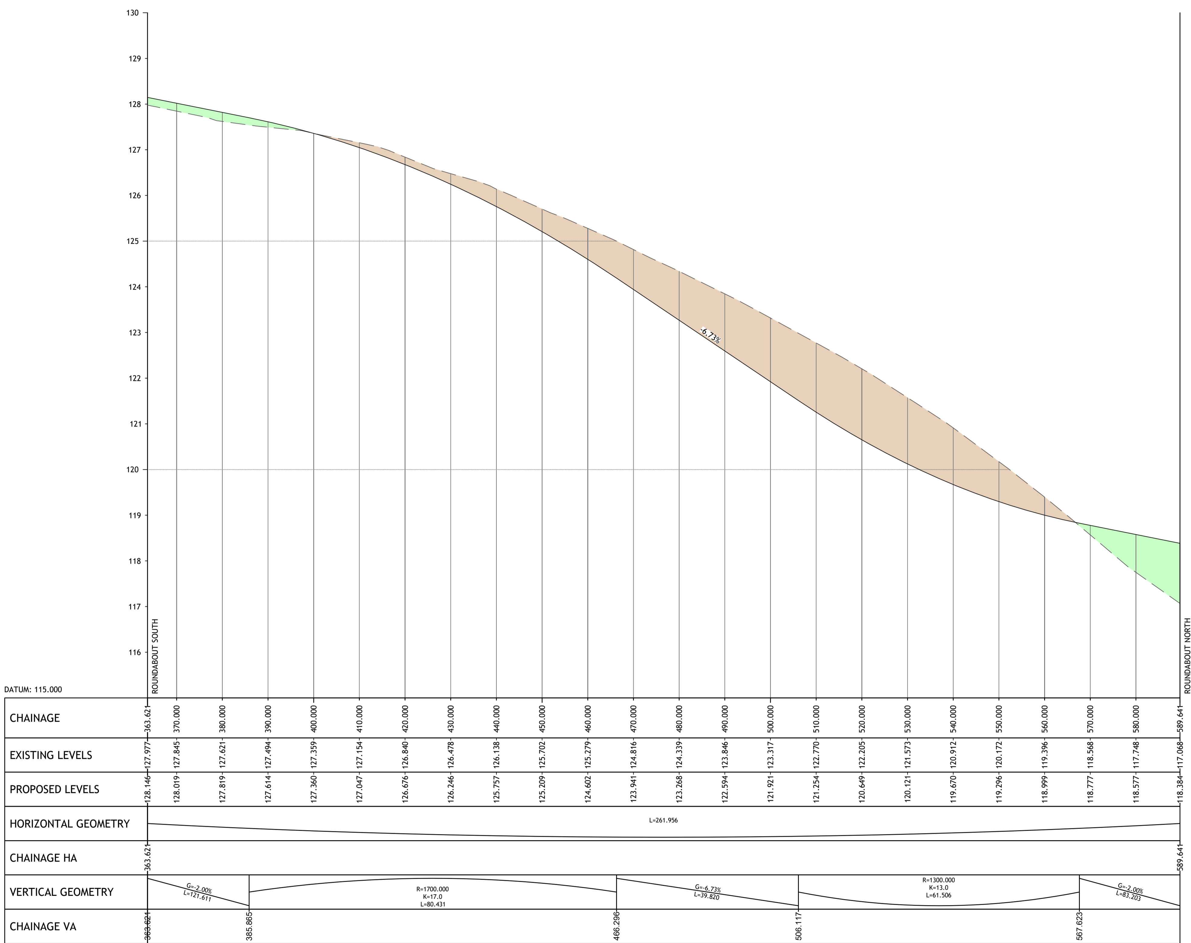
PROFILE NAME: LINK ROAD SECTION B SCALE: H 1:500, V 1:50
