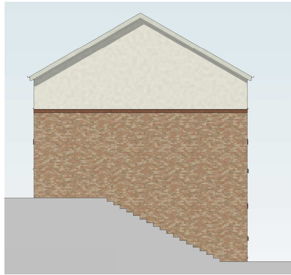
6 | HTA3 SIDE_Elevation 1 : 100
