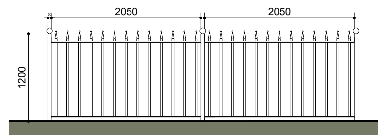
1.2m metal railing
