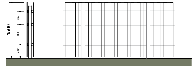
Section Elevation
