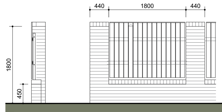
1.8m high brick wall with timber fence panel
