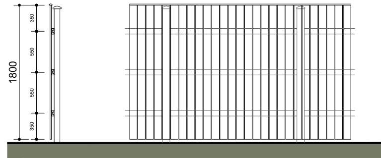
Section Elevation
