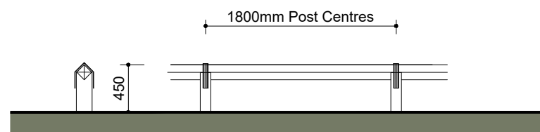
Section Elevation
