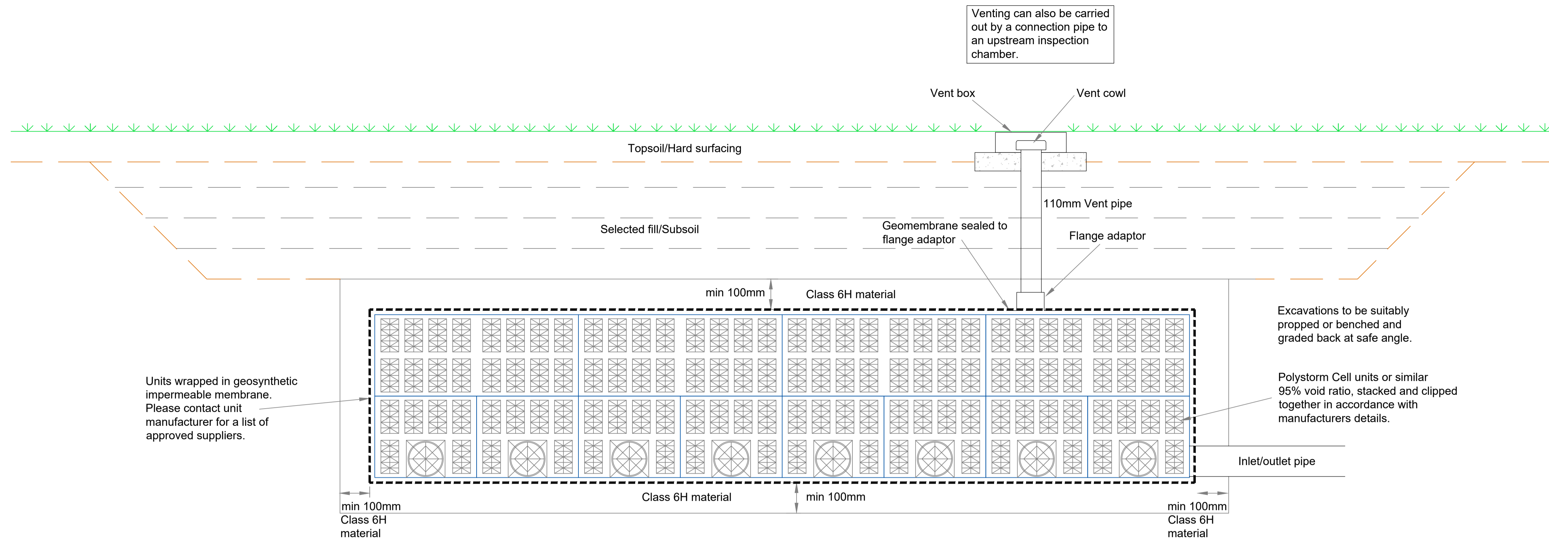
Typical Offline Cell Unit Attenuation tank
