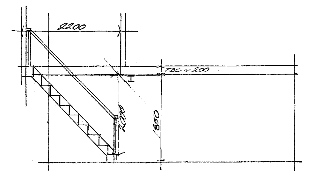
CELLAR SECTION
