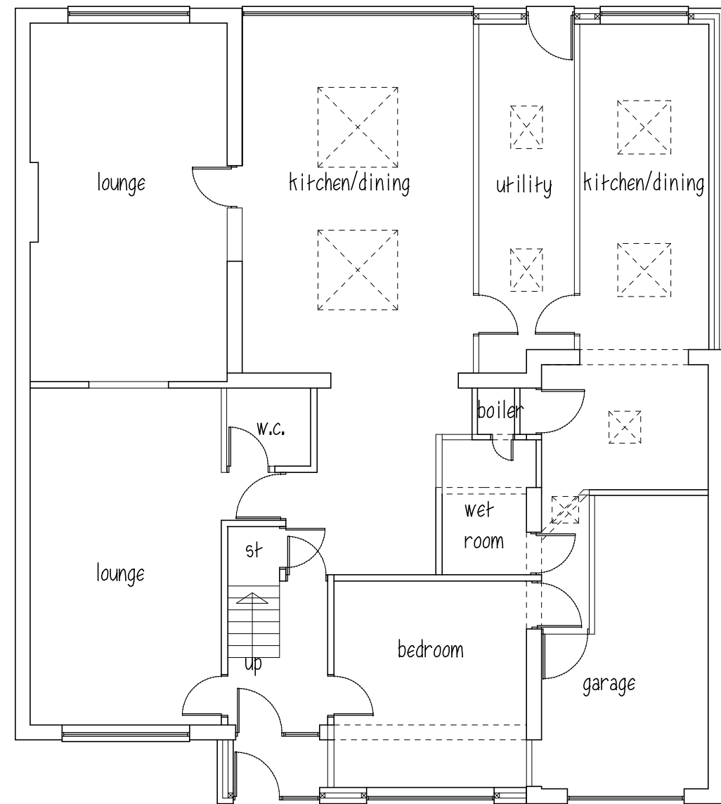
GROUND FLOOR
