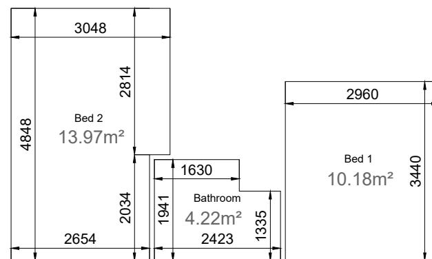
First Floor. 1 : 100
