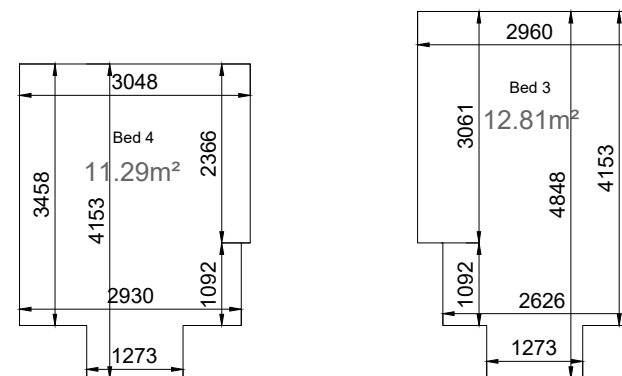
Second Floor. 1 : 100
