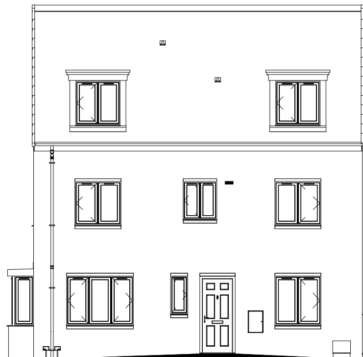
Front Elevation. 1 : 100
