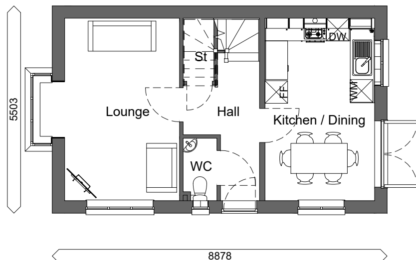
Ground Floor. 1 : 100
