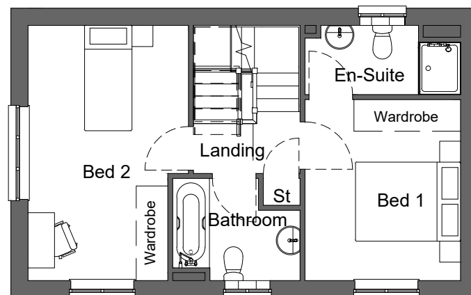
First Floor. 1 : 100
