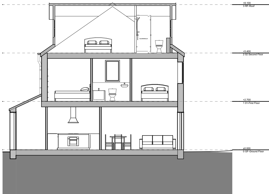
3 Section CC 1:100
