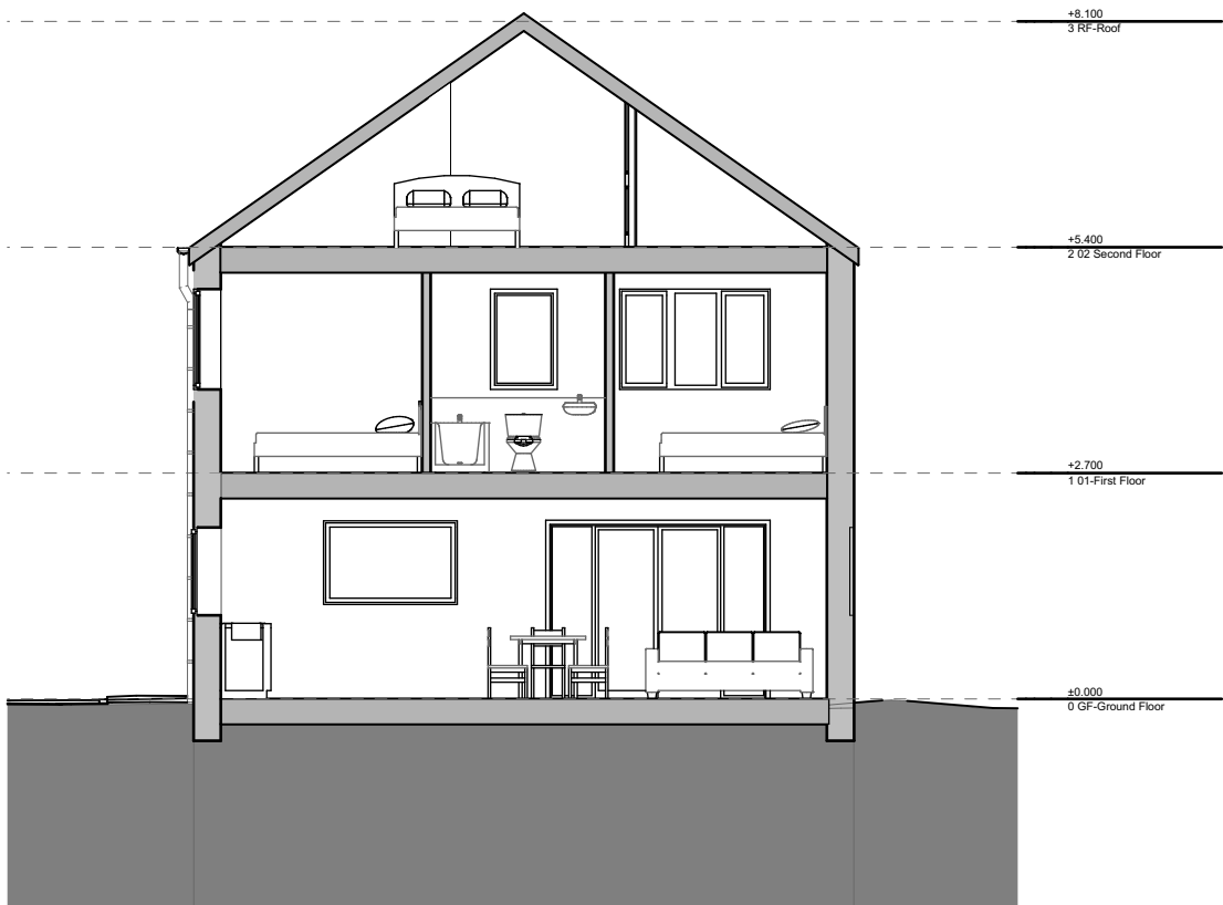
1 Section AA 1:100
