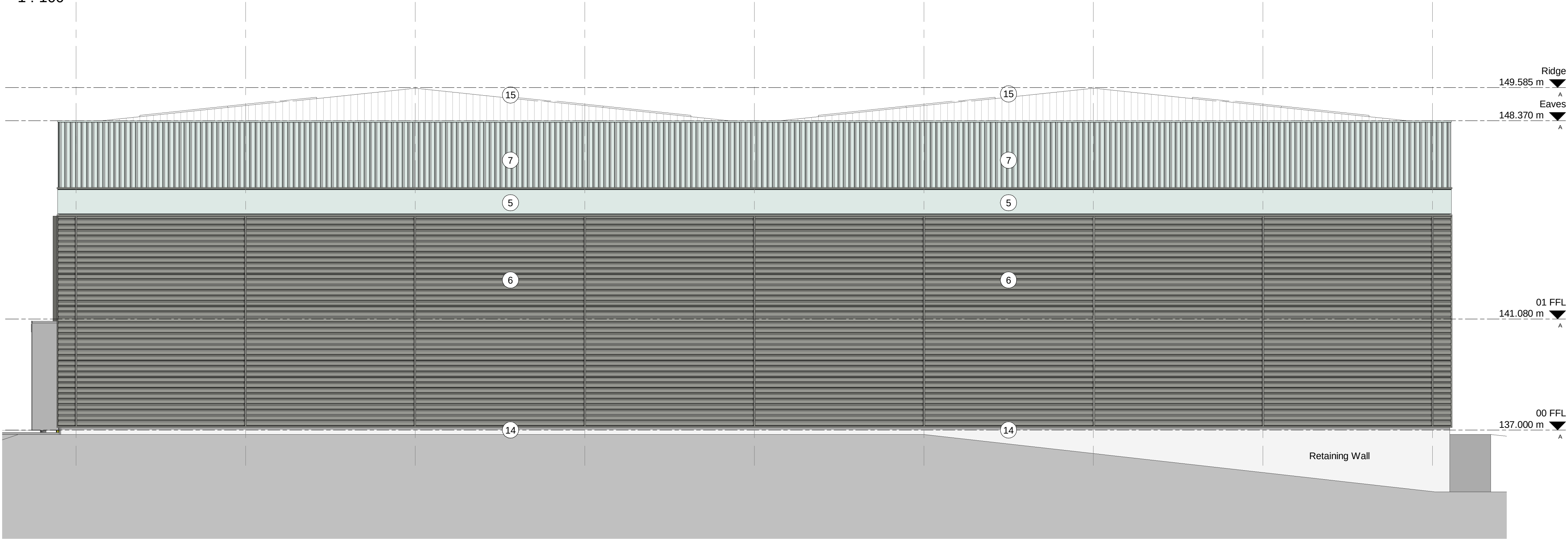
North East Elevation 1 : 100
