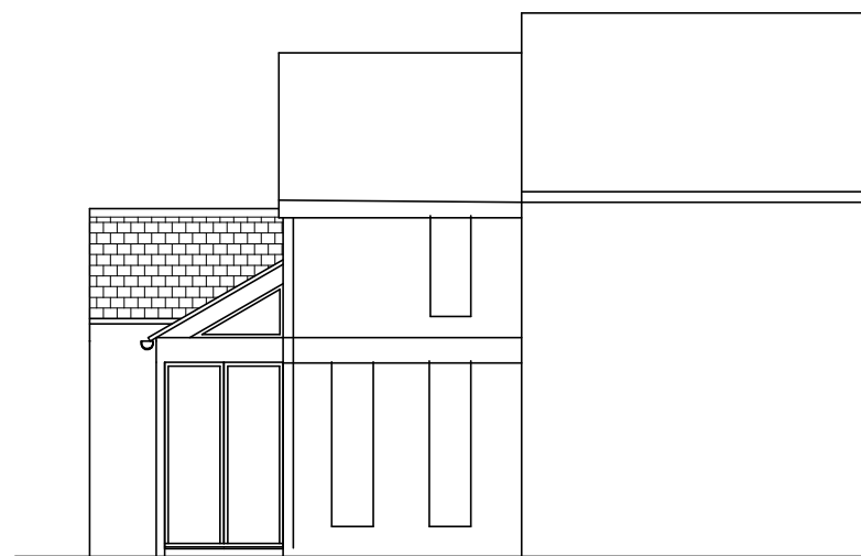
SOUTH ELEVATION
