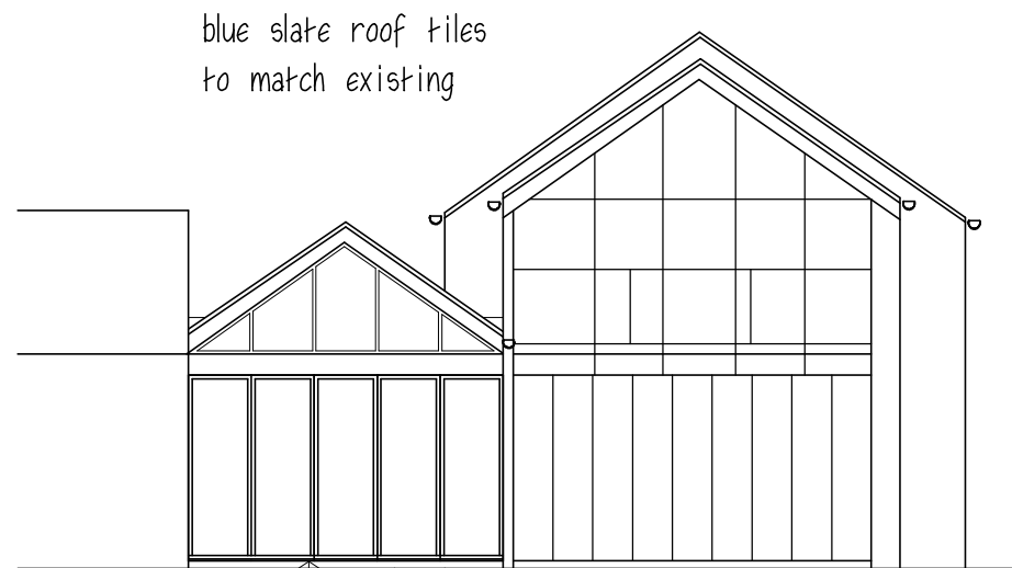
WEST ELEVATION
