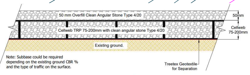
Figure 4: Indicative Cellweb TRP system with overfill:
