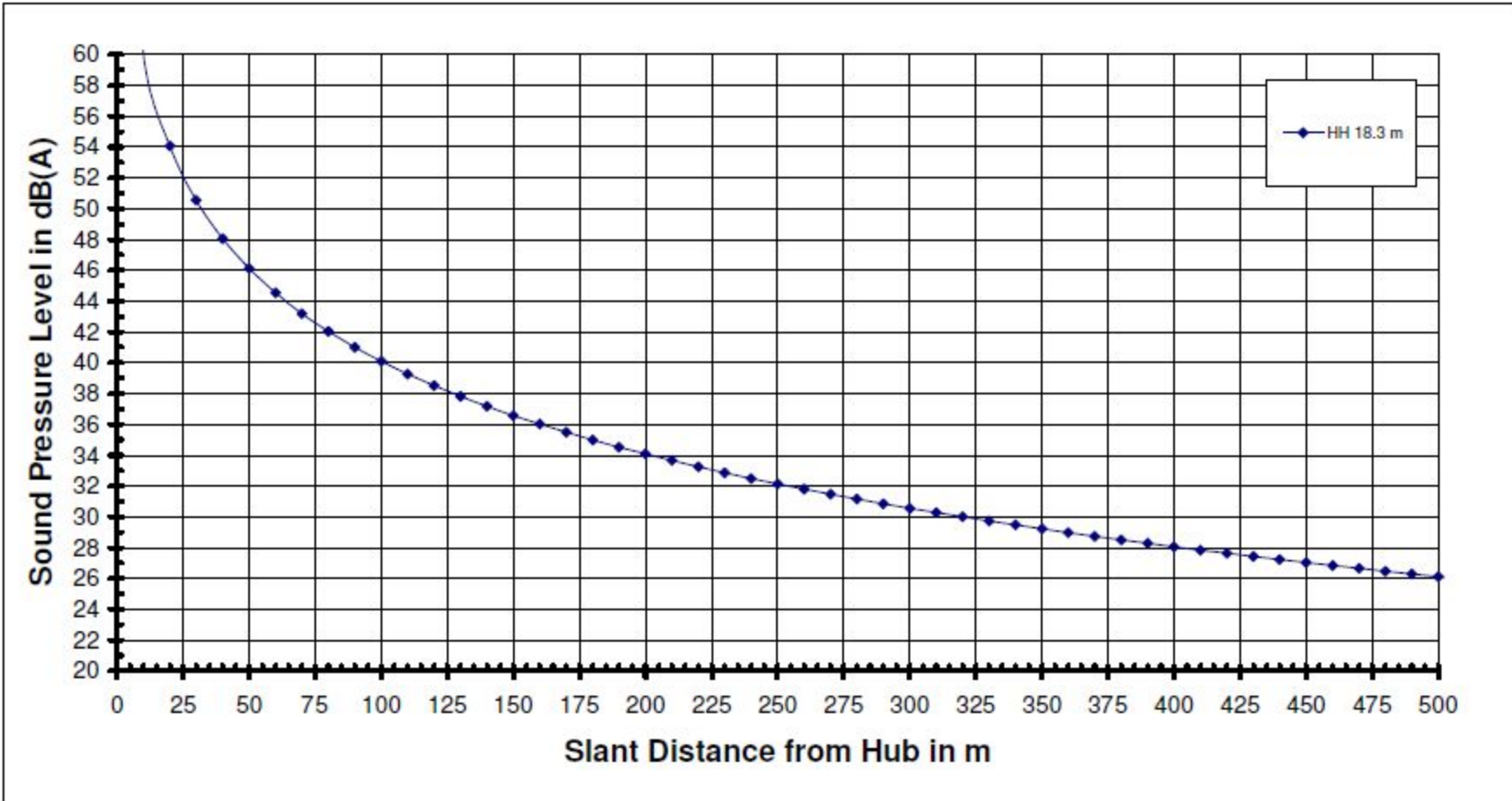
Sound Pressure Level (according to BWEA Small Wind Turbine Performance and Safety Standard) of a Gaia-Wind 11 kW with 18.3 m Hub Height depending on Slant Distance (Reference: 8 m/s at Rotor Centre Height)
