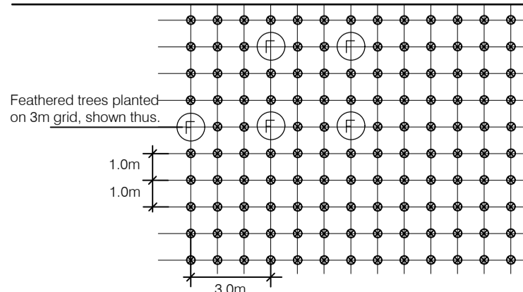
WOODLAND EDGE THICKET MIX - LAYOUT GRID 1:200
