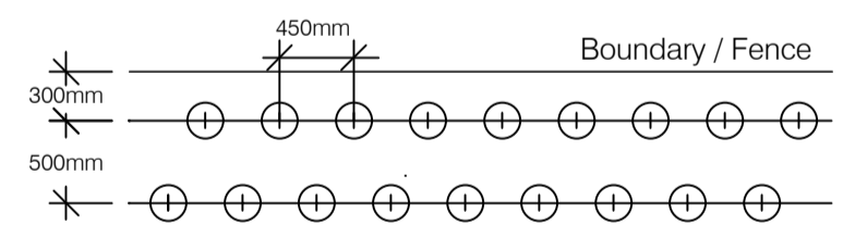
HEDGE PLANTING DETAIL 1:50
