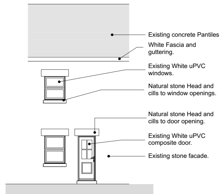
EXISTING REAR 1:100
