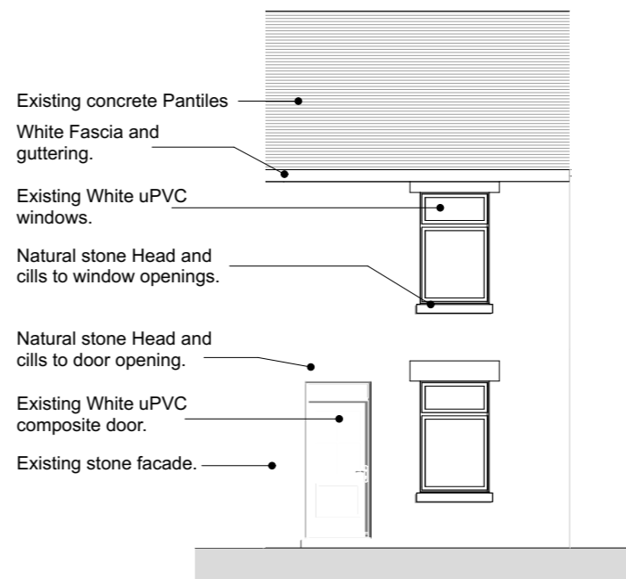
EXISTING FRONT 1:100
