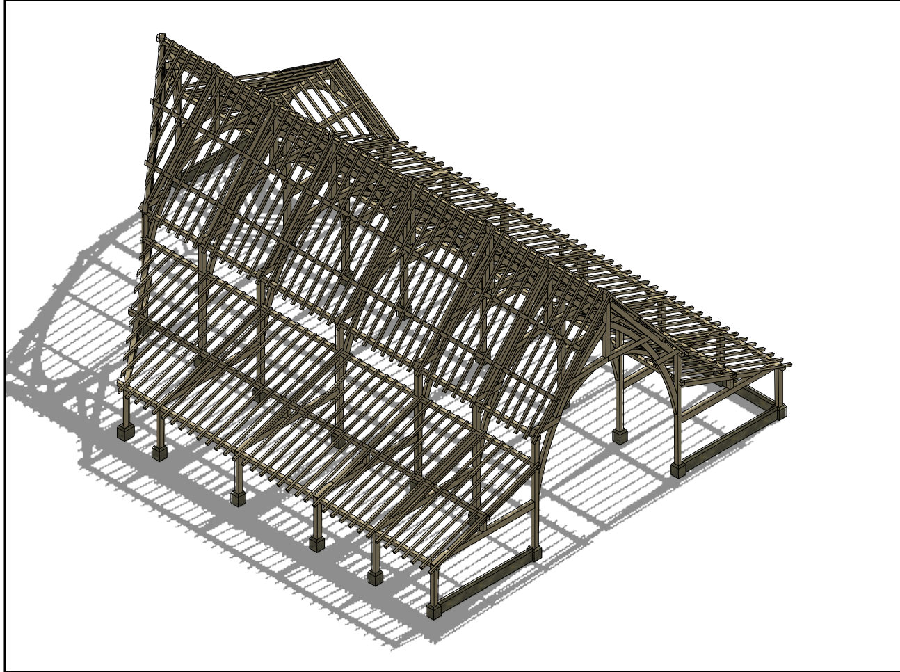
ISOMETRIC OF FRAME (FACING SOUTHWEST)
