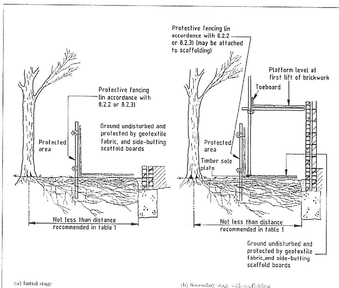
Figure 6. Scaffolding within a protected area (see 8.3.2)
