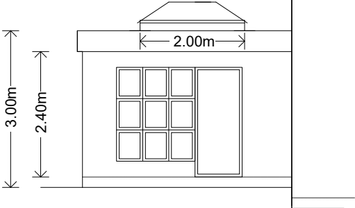
SIDE ELEVATION B
