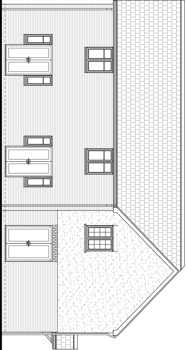
REAR ELEVATION
