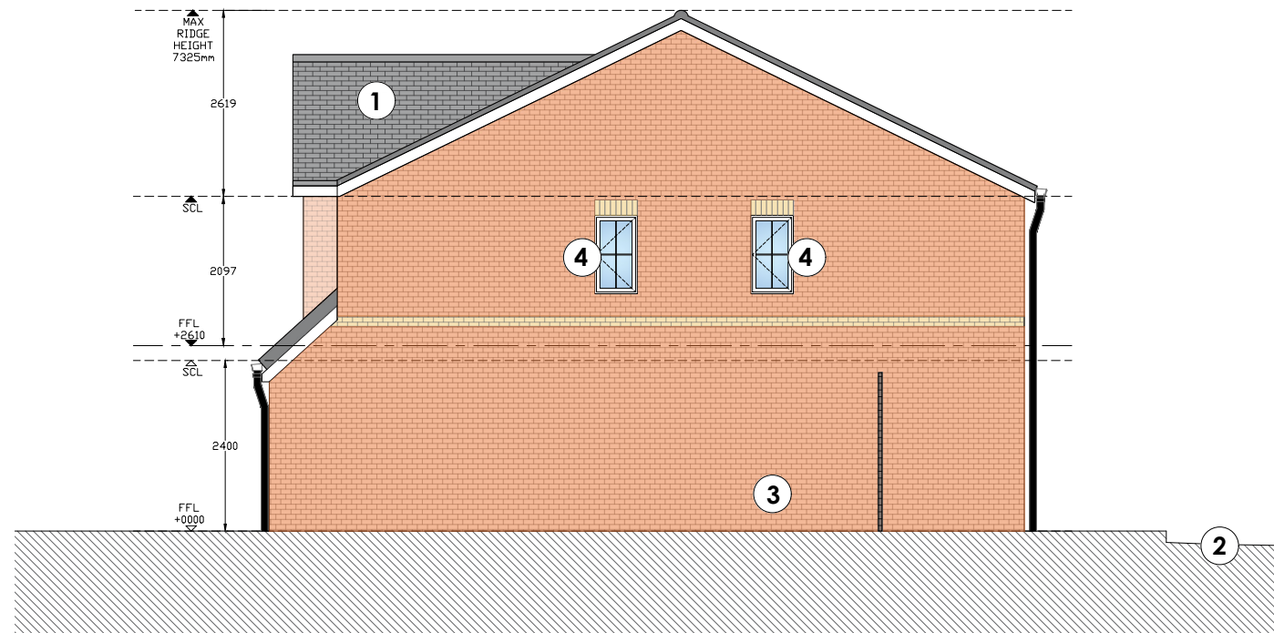
Elevation 04: Proposed Side Elevation
