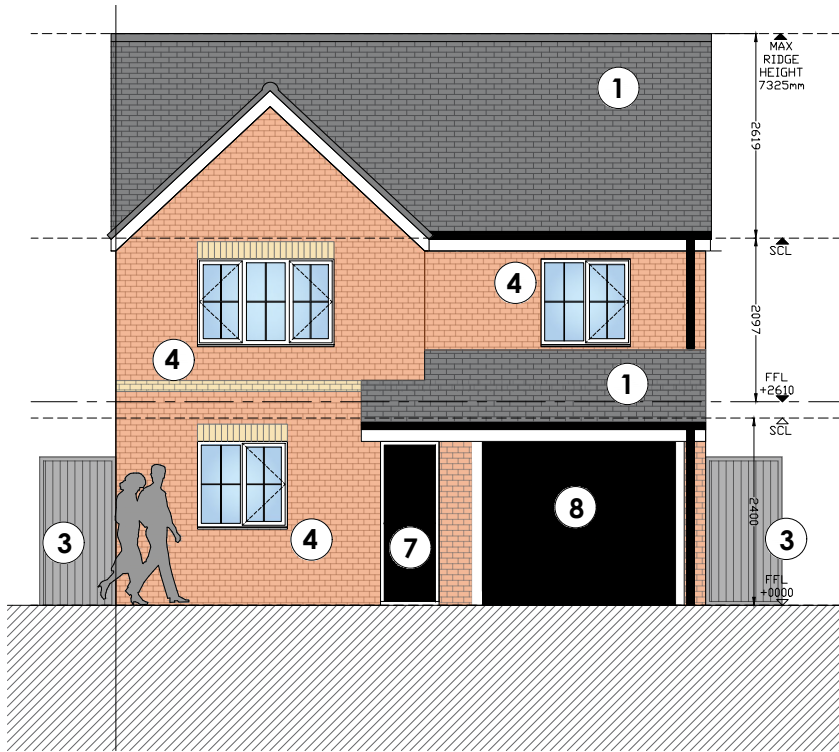
Elevation 01: Proposed Front Elevation
