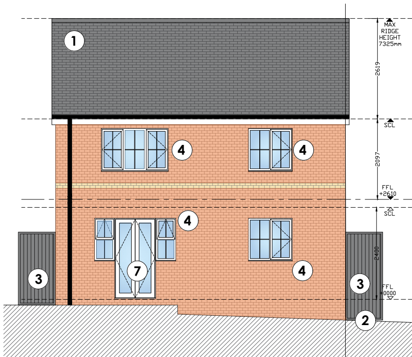
Elevation 03: Proposed Rear Elevation
