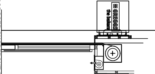
PROPOSED SHOPFRONT SECTION
