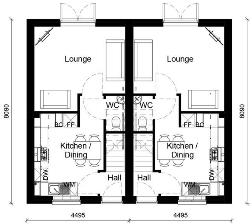
Ground Floor. 1 : 100
