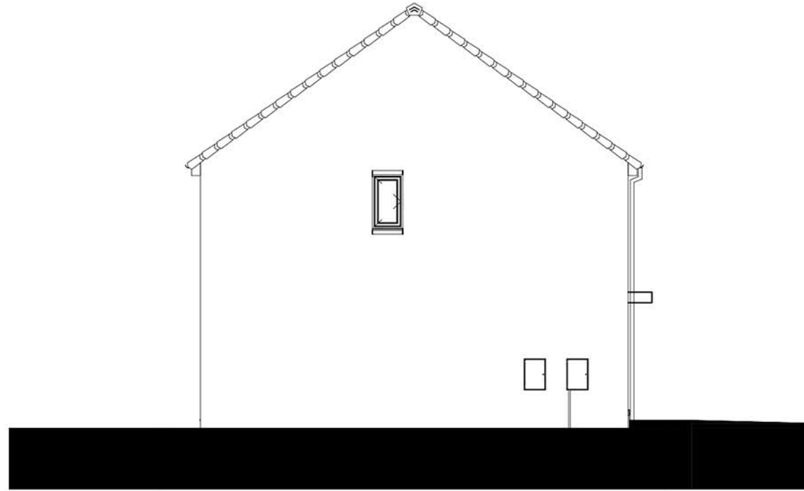
Left Elevation. 1 : 100
