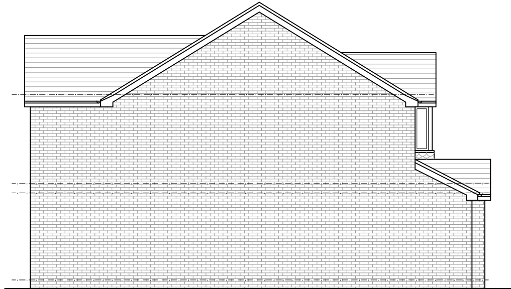
NORTH ELEVATION
