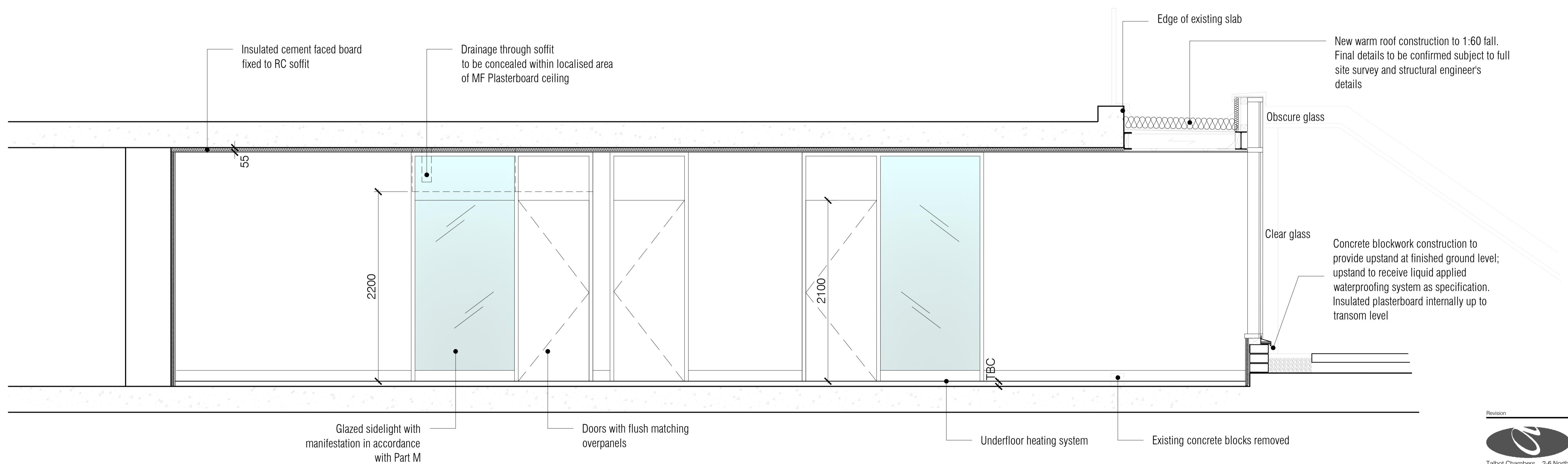
SECTION B-B
