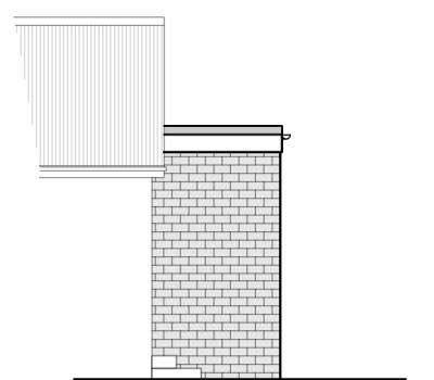
Proposed (Part) Side Elevation
