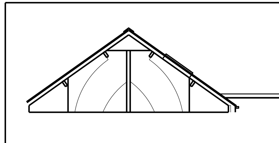
Cross Section / West Elevation - Existing
