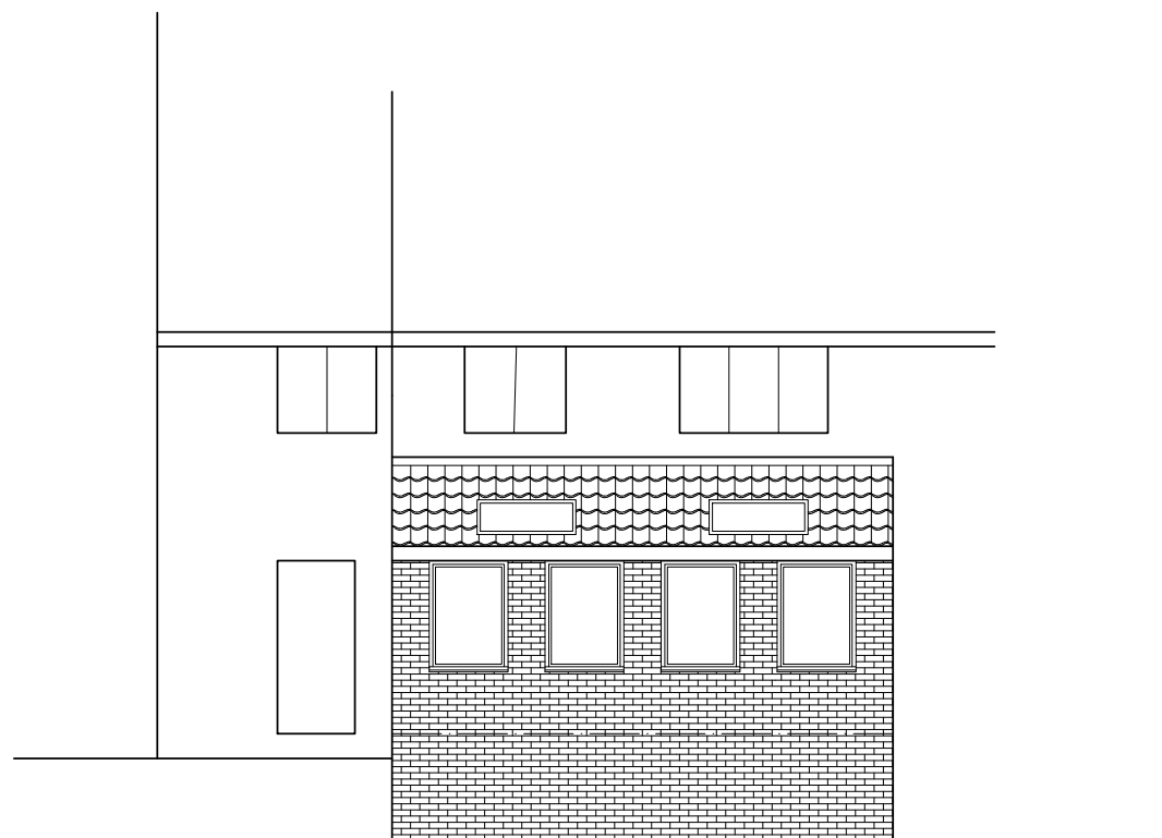
REAR ELEVATION
