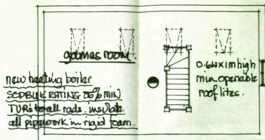
First Floor layout.
