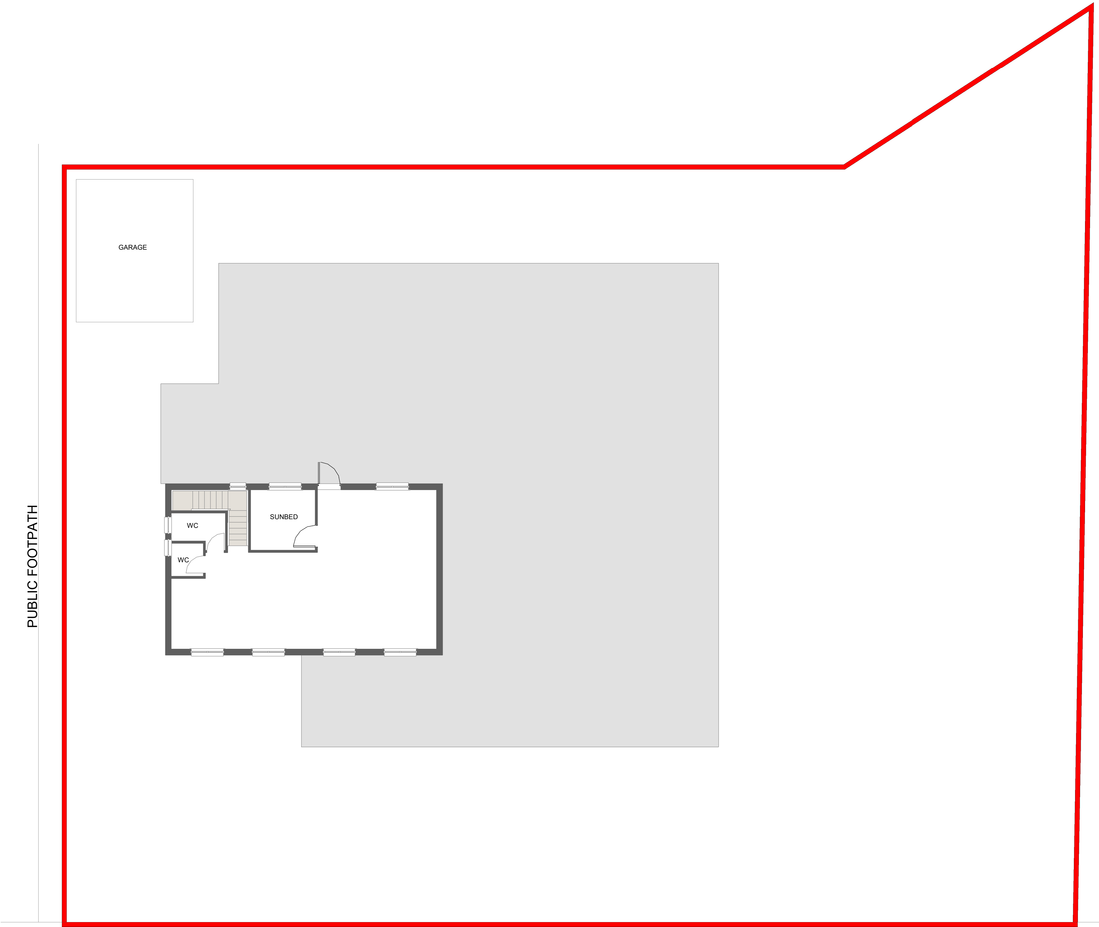
Existing First Floor 1 : 100
