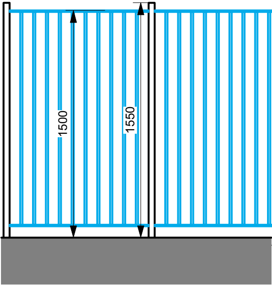
1500mm high metal railings. Colour - Black 300 x 50mm concrete pin kerb laid flat below.
