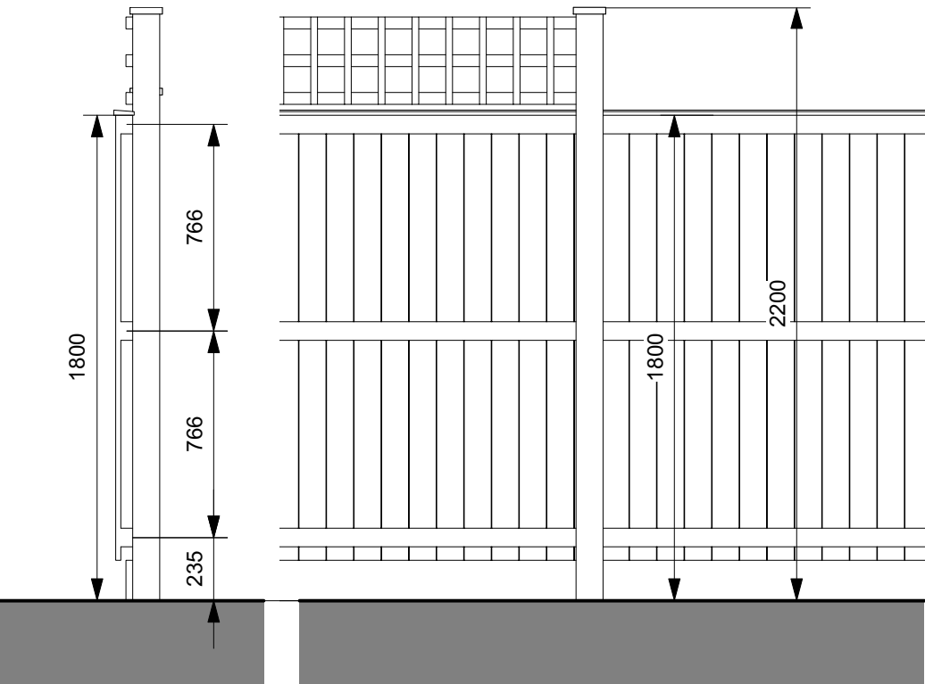
1.8m high close boarded timber fence. Posts 100 x 100mm Rails 44 x 69mm. Boards 19 x 120mm. Gravel board 25 x 150mm. Weathered capping 69 x 32mm.
