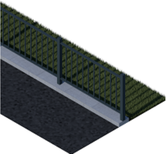
550mm high metal railings. Colour - Black 300 x 50mm concrete pin kerb laid flat below.
