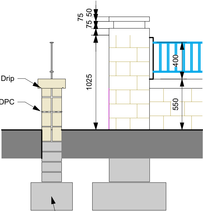
Foundations to engineer's detail Stone wall with artstone capping
