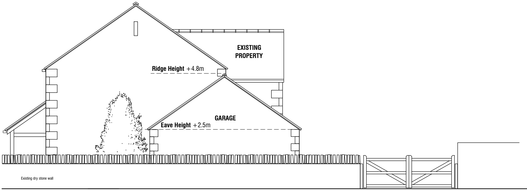
REAR ELEVATION 1:100
