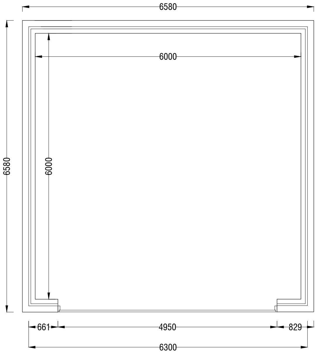
FLOOR PLAN 1:50
