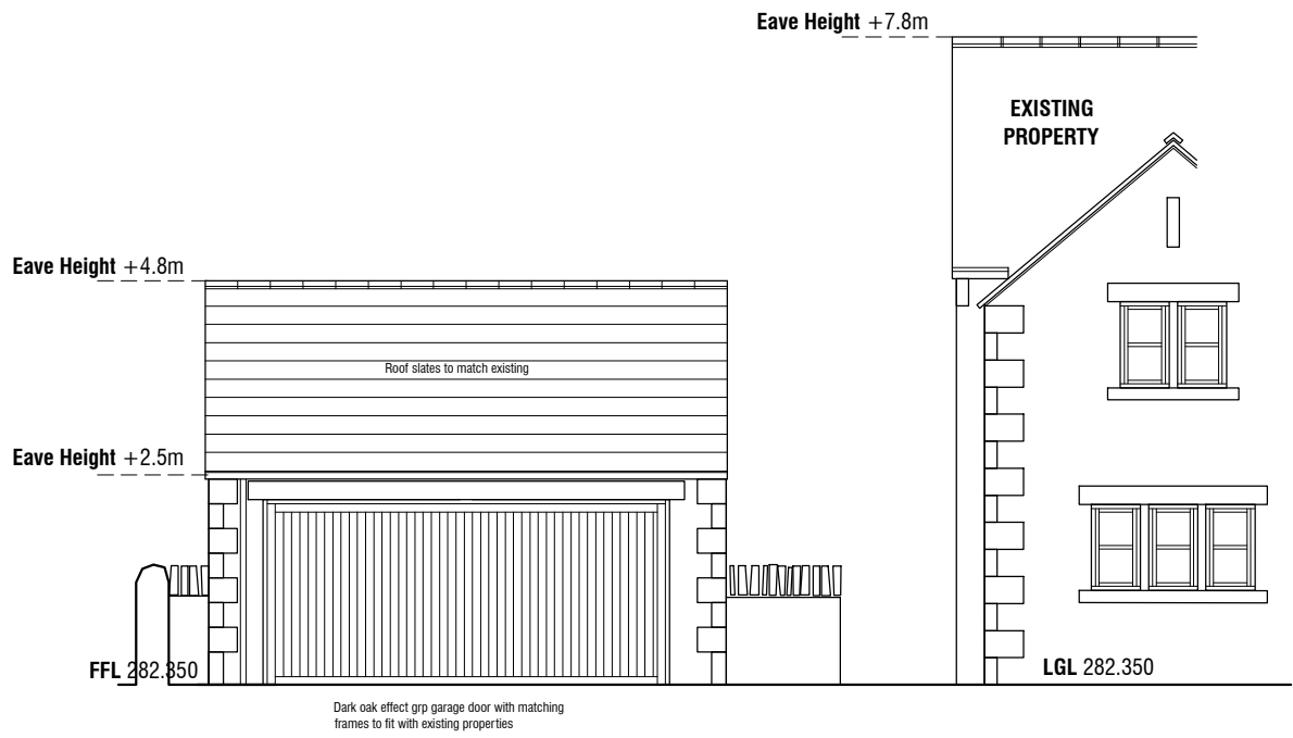
REAR ELEVATION 1:100
