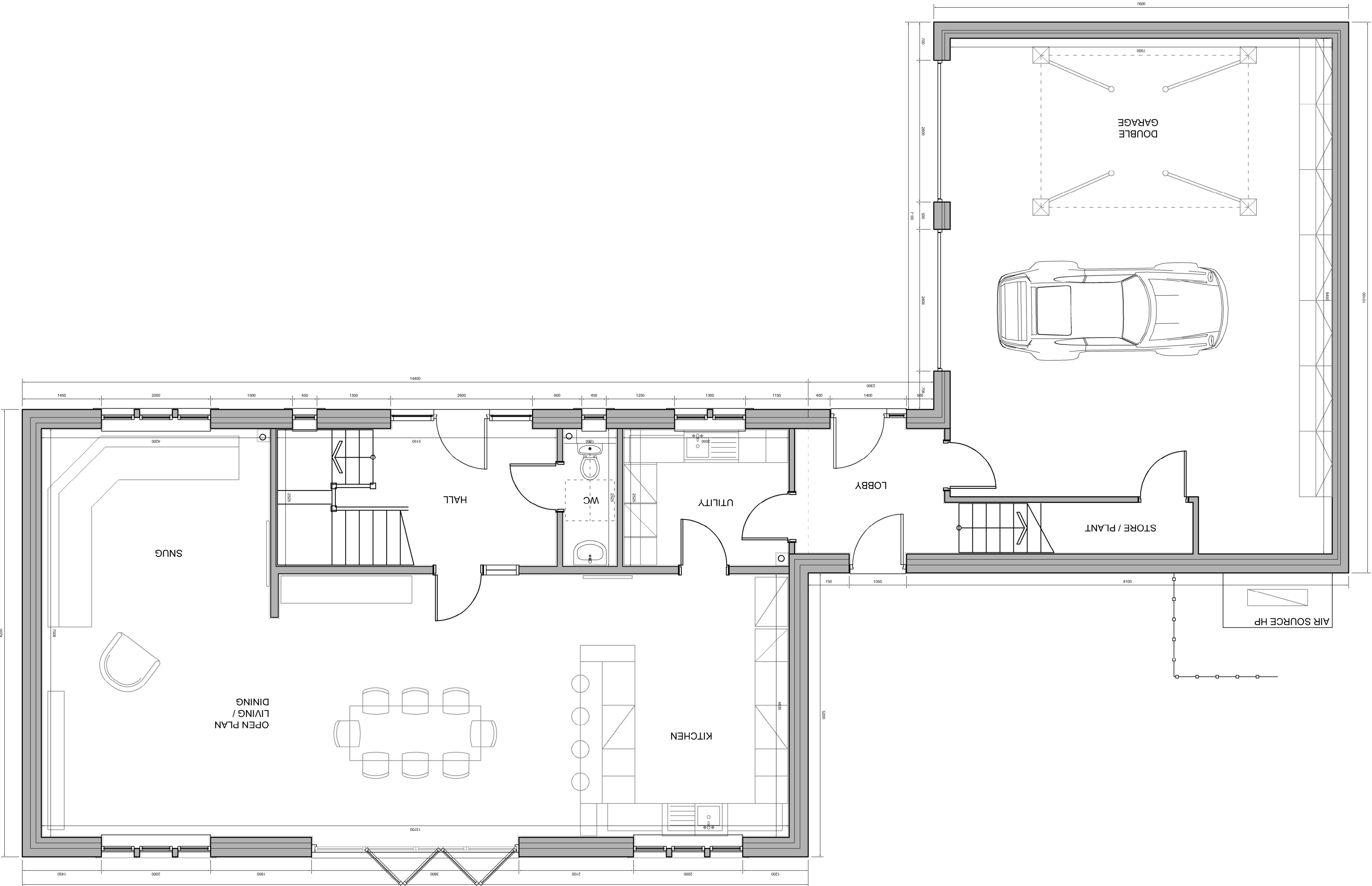
GROUND FLOOR | 1:50 @ A1
