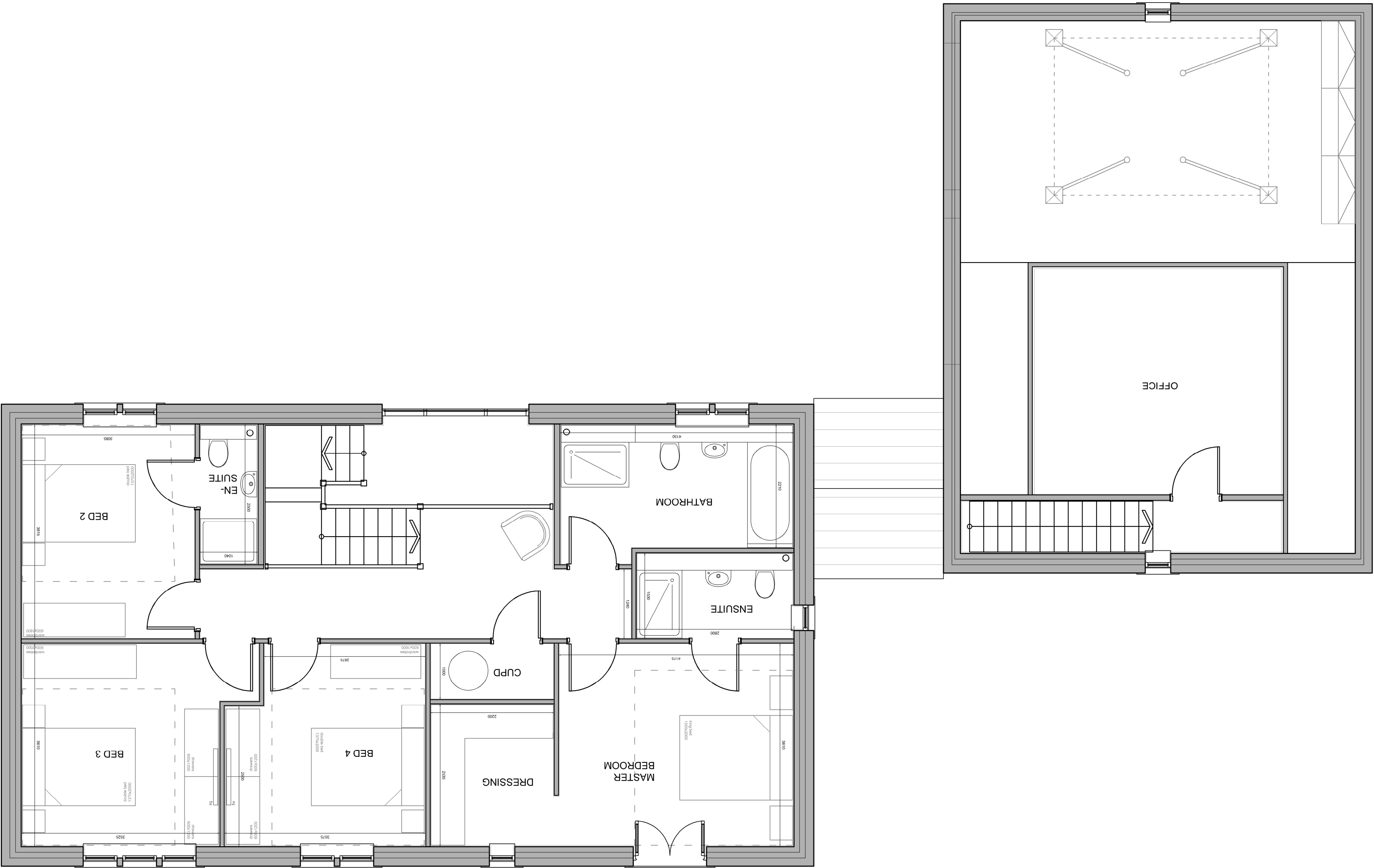
FIRST FLOOR | 1:50 @ A1
