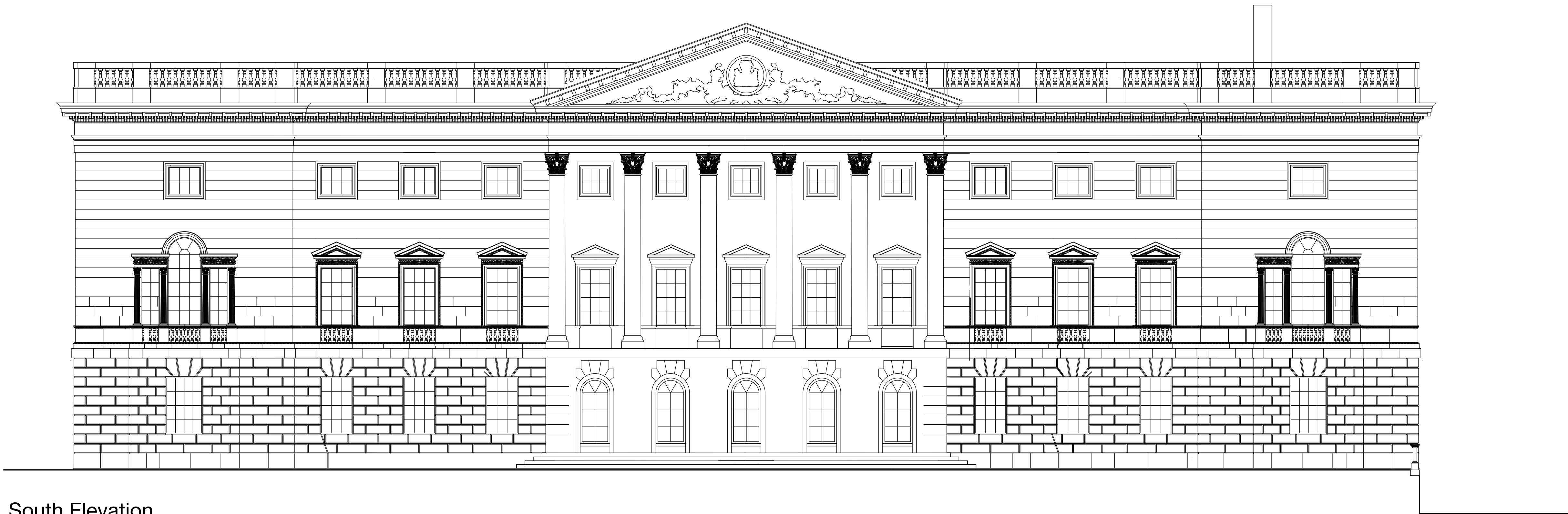
South Elevation
