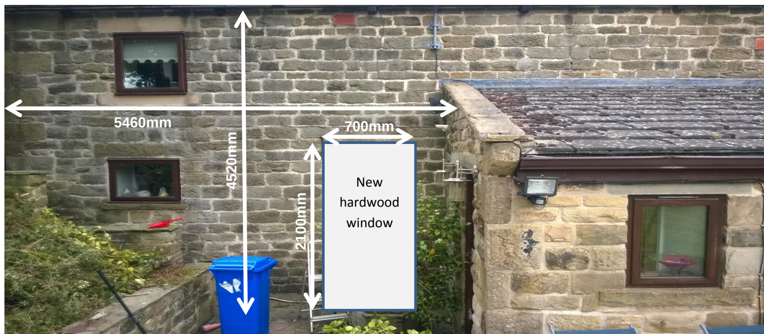
Fig 1 – Rear Elevation
