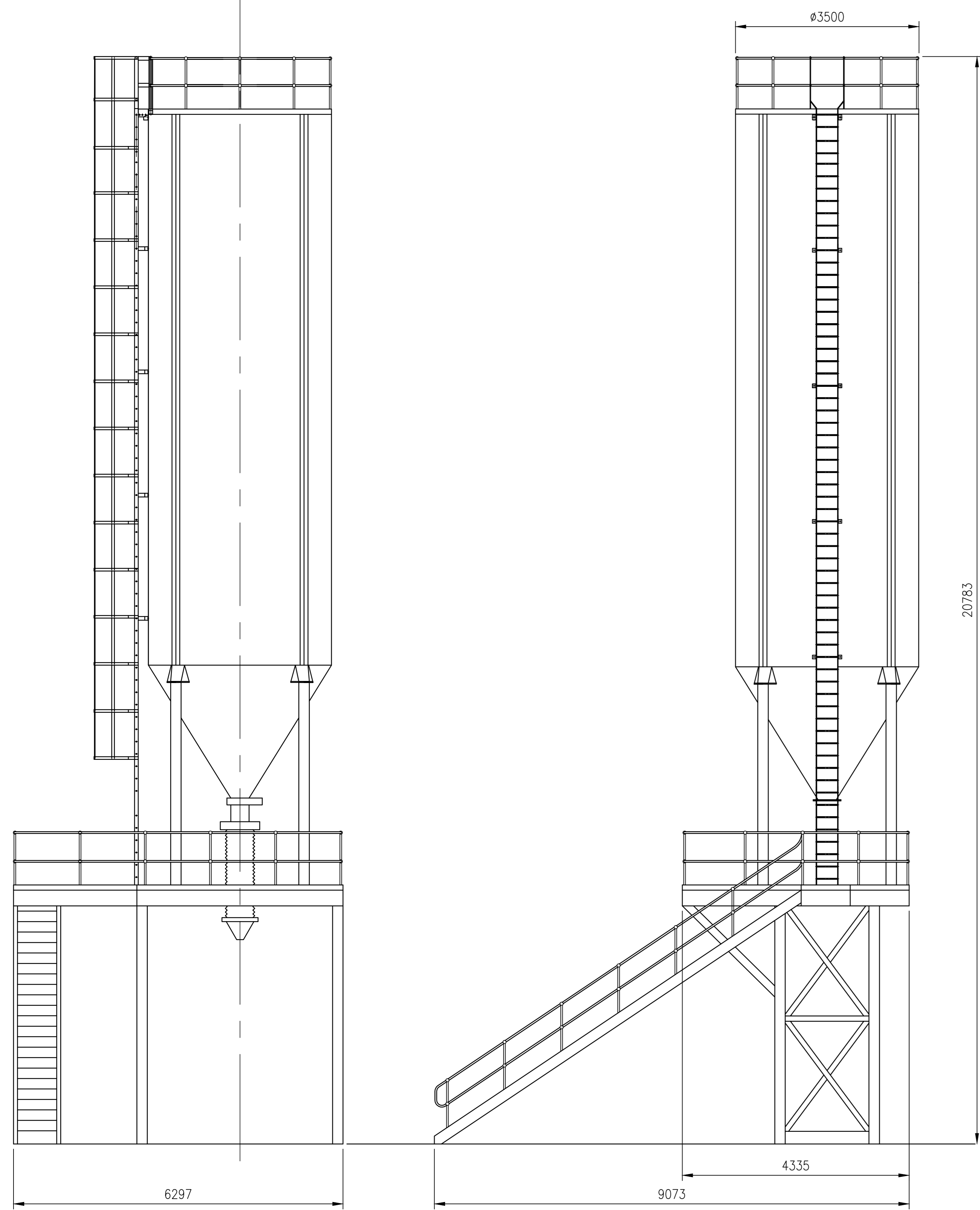
PROPOSED SILO SCALE ~ 1:50 @ A0
